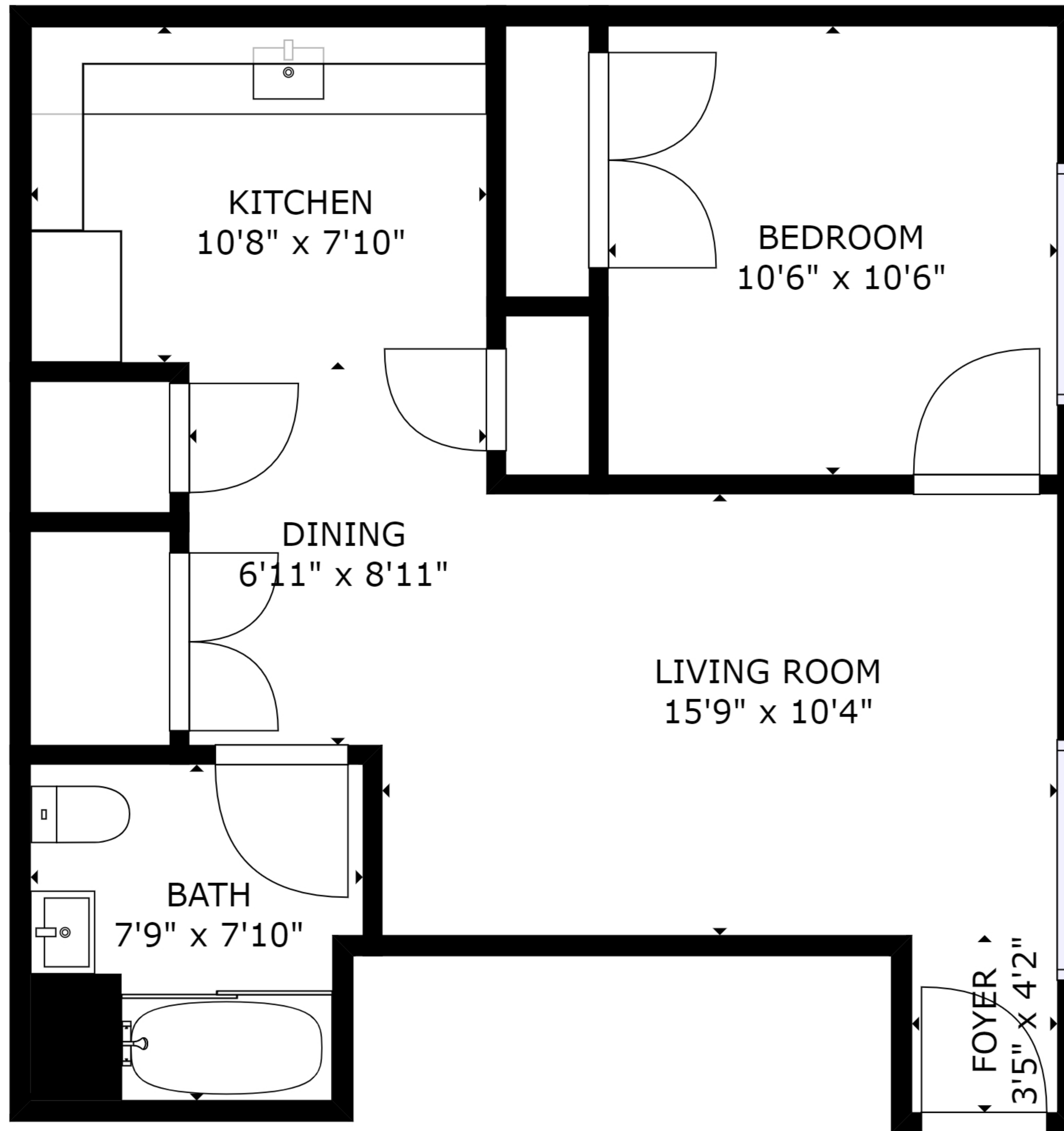
FLOOR 1
